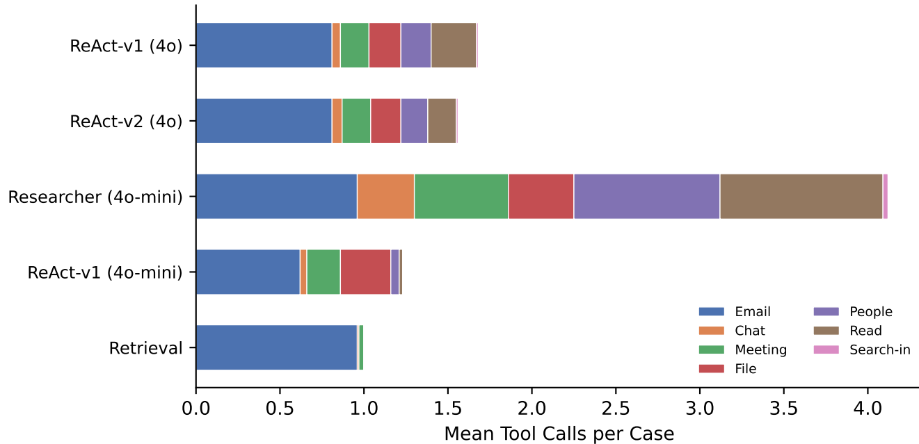
Tool Usage Breakdown
