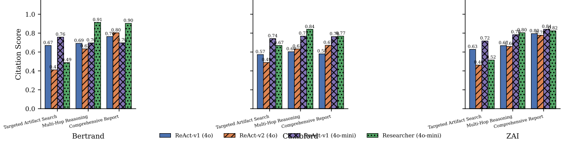
Fig. 13. Mean citation score by query type and tenant. RESEARCHER (4o-mini) leads on comprehensive report queries where its planning stage systematically covers multiple source types, while the reactive configurations are competitive on targeted artifact search queries.
