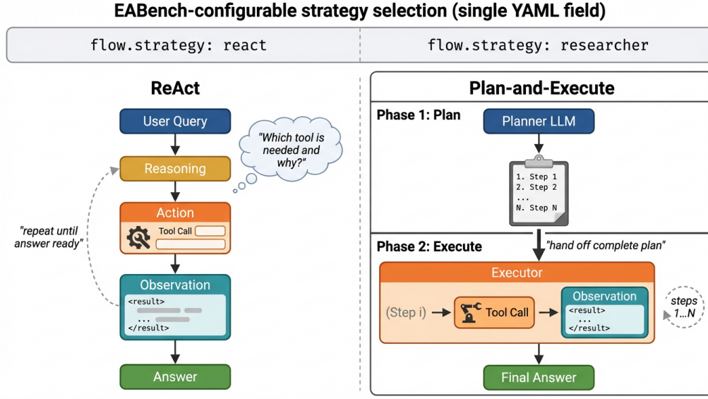
Fig. 5. The two cognitive architectures natively supported by EABench as hot-swappable flow.strategy values. ReAct (left) interleaves reasoning and acting in a tight feedback loop; Plan-and-Execute (right) separates a global planning phase from sequential step-wise execution, reducing context drift on long multi-hop tasks.
