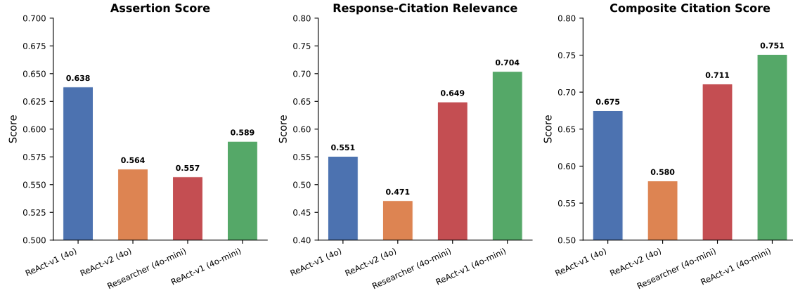
Fig. 8. Weighted-aggregate metrics across all tenants. Left : assertion score—REACT-v1 (4o) leads (0.638). Middle : response-citation relevance—REACT-v1 (4o-mini) leads (0.704). Right : composite citation score (mean of TS-Rel and RC-Rel)—REACT-v1 (4o-mini) leads (0.751).
