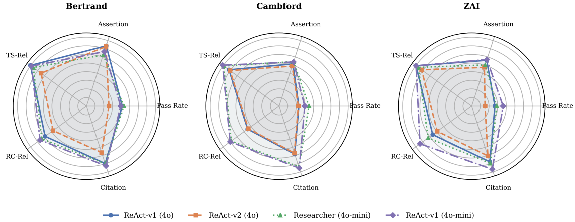
Fig. 11. Per-tenant configuration profiles. Each subplot shows the four evaluated configurations on a shared radar for one tenant. On Bertrand (dense, small) all configurations overlap; on Cambford (temporal multi-hop) RESEARCHER (4o-mini)’s citation and pass-rate advantage widens; on ZAI (large, bursty) REACT-v1 (4o-mini) matches or exceeds the planner on assertion accuracy.
