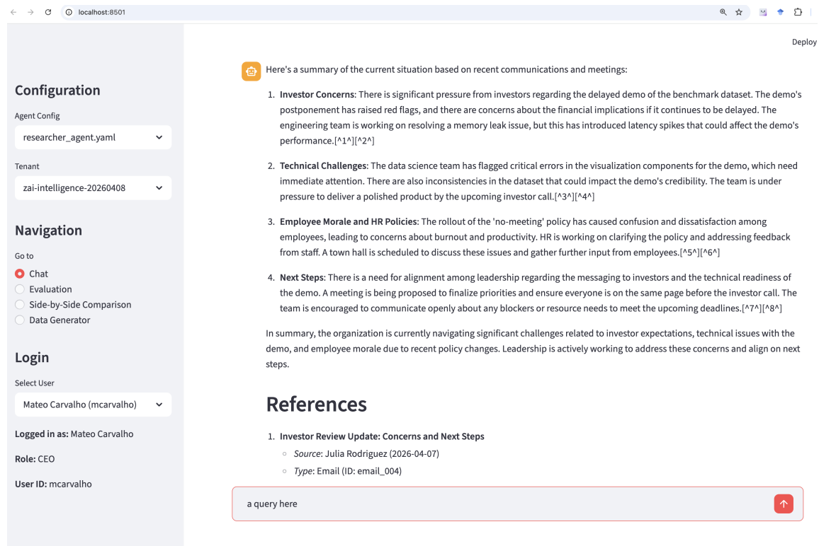
Fig. 7. EABench interactive chat interface. The left sidebar provides configuration controls (agent strategy, tenant, and user persona); the main panel displays the agent’s structured response with inline citation markers and a references section listing source artifacts with metadata. A query input box at the bottom enables iterative exploration under the selected persona.
