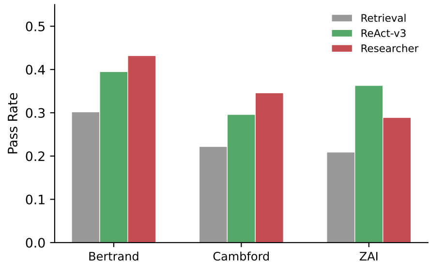
Snippet-Only vs. Browsing
