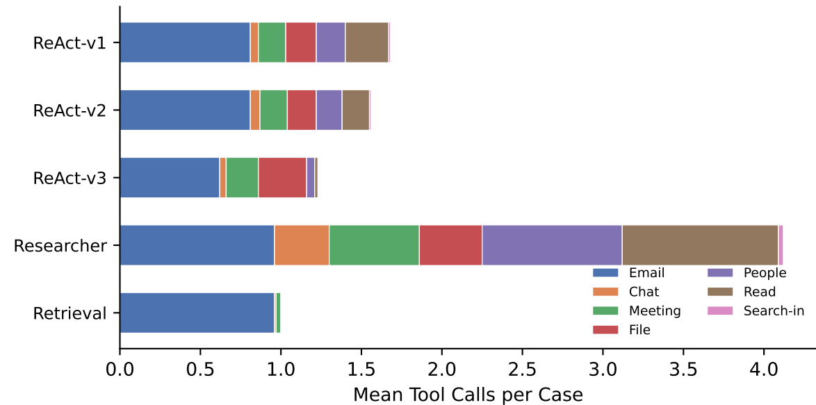
Tool Usage Breakdown
