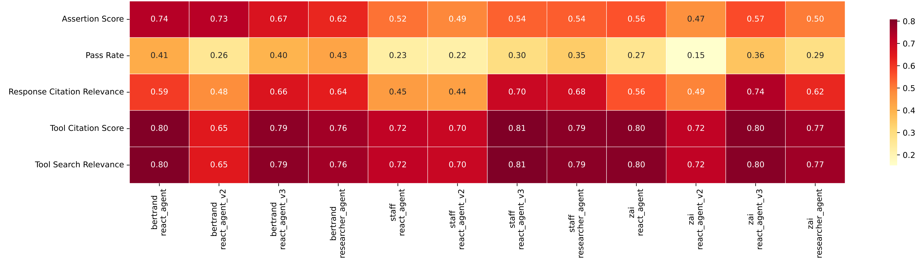
Key Metrics Heatmap (Tenant × Agent)
