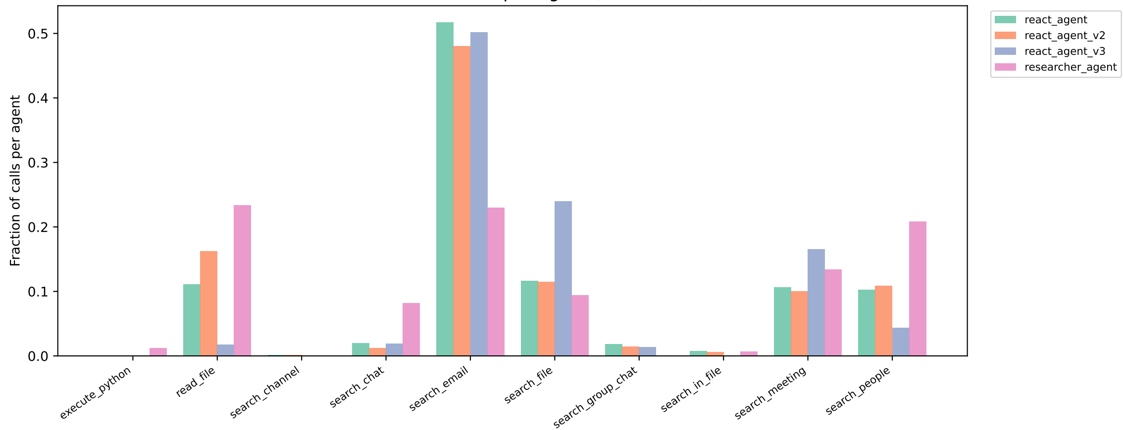
Tool Call Distribution per Agent (Normalized)
