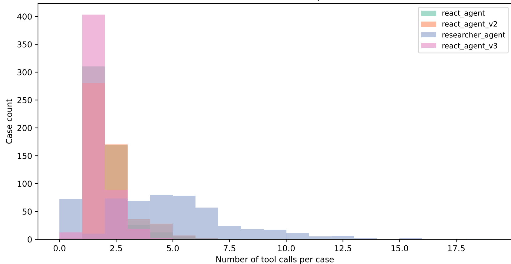
Distribution of Tool Calls per Case
