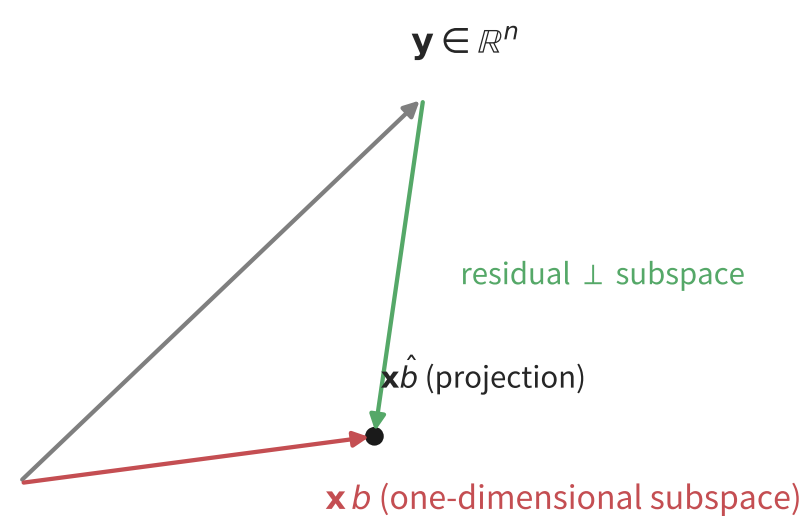
(c) Geometry: least squares = orthogonal projection
