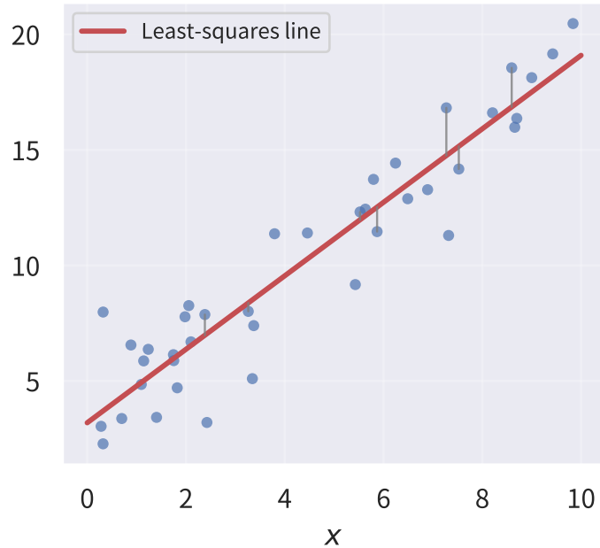
(a) Fitting: minimum sum of squared residuals
