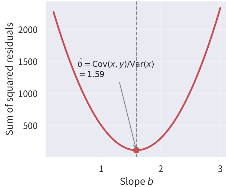
(b) Objective: unimodal and tractable
