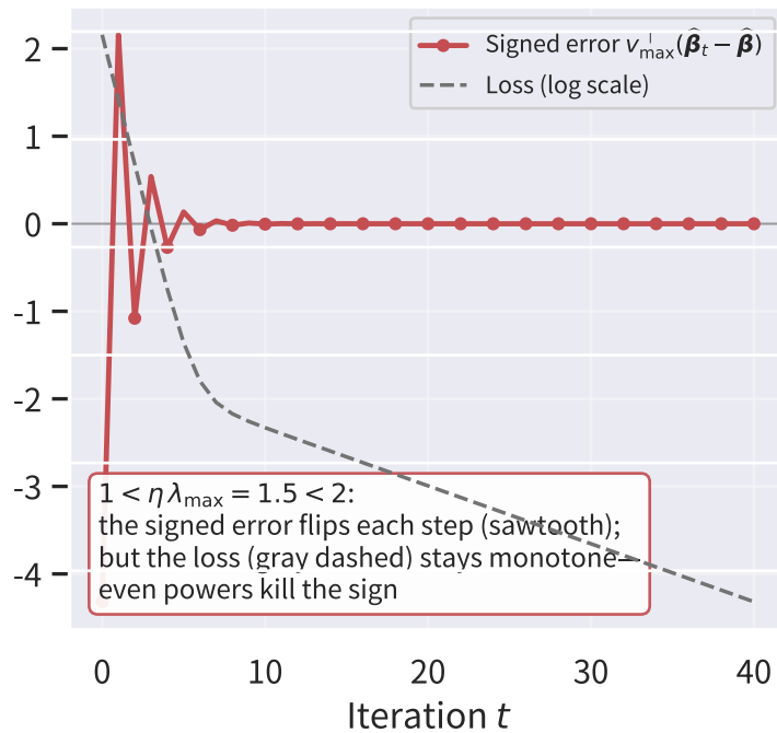
(b) Oscillating decrease: \eta = 1.5
