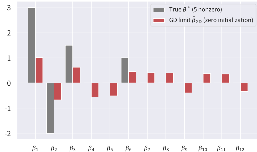
(a) GD automatically finds the 'energy-concentrated' interpolating solution
