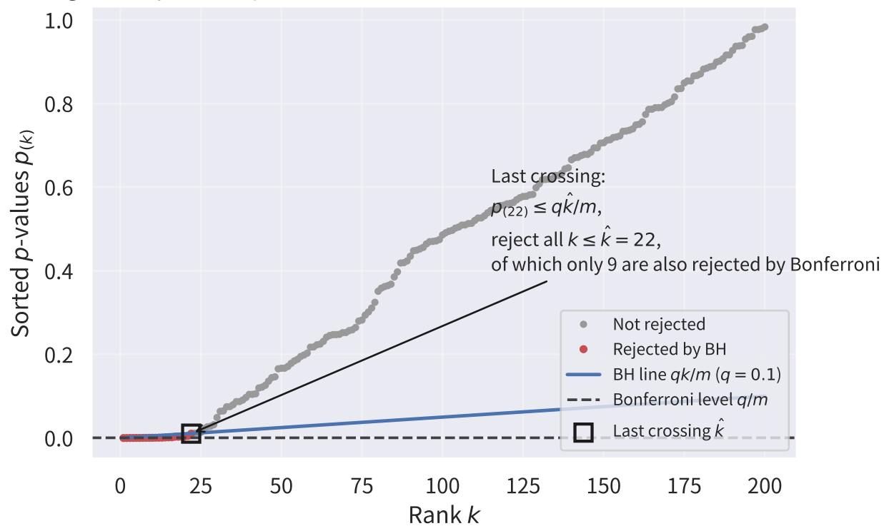
(a) BH geometry: the sloped line relaxes the threshold; Bonferroni is a horizontal line
