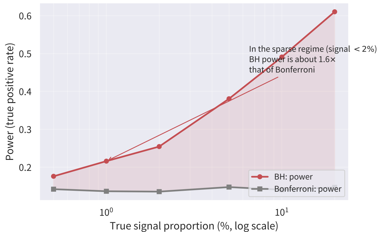
(b) Power comparison ( m = 1000 , q = 0.05 , 200 replications; FDR of both methods stays below q )
