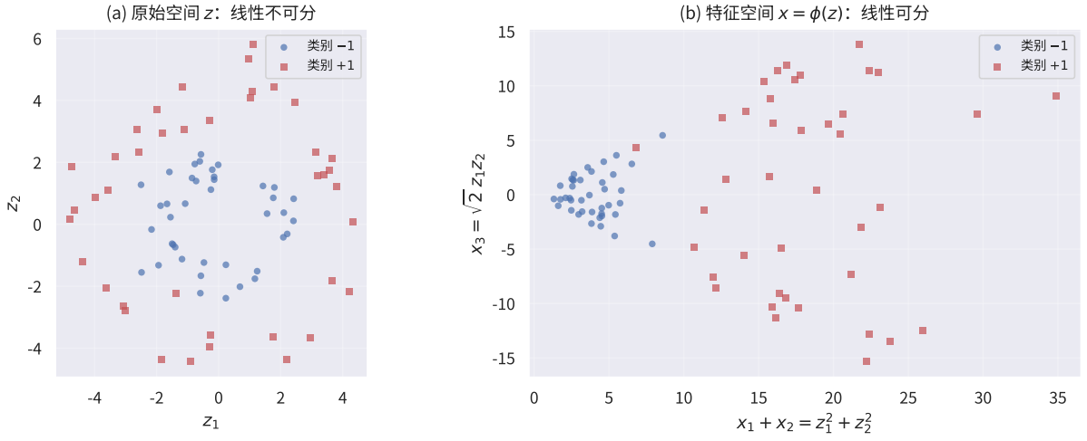
图 10: The geometric essence of kernel methods: the same ring-shaped data (two classes by radius) cannot be separated by any straight line in the original latent space \mathbf{z} (left); lifted by the quadratic feature map \phi(\mathbf{z}) = (z_1^2, z_2^2, \sqrt{2}z_1z_2) into feature space (right), a single linear function separates them. Linear in \mathbf{x} = nonlinear in \mathbf{z} — and hence the prediction of linear regression becomes a natural nonlinear method in latent space.
