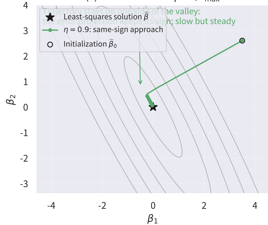
(a) Monotone: 0 < \eta \leq 1/\lambda_{\max}
