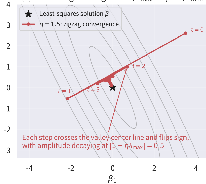
(b) Oscillating convergence: 1/\lambda_{\max} < \eta < 2/\lambda_{\max}
