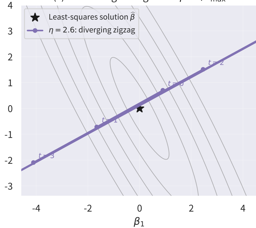
(c) Oscillating divergence: \eta \geq 2/\lambda_{\max}
