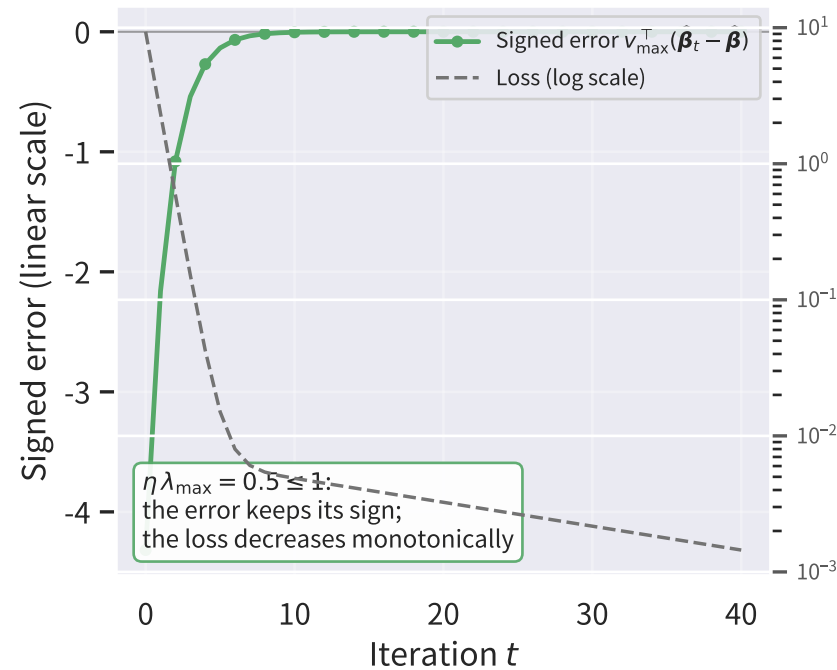
(a) Monotone decrease: \eta = 0.5
