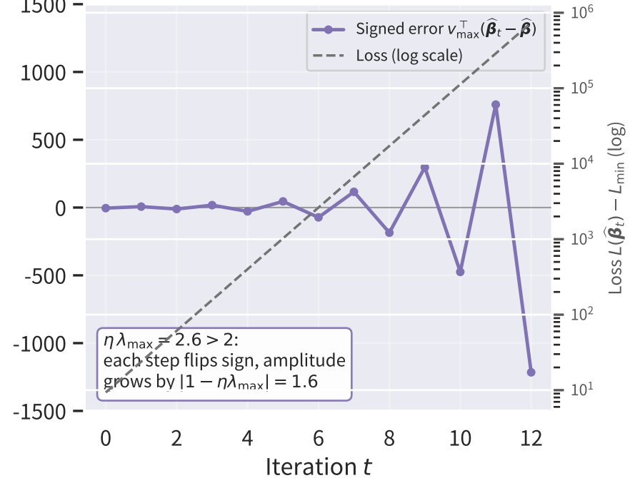
(c) Oscillating divergence: \eta = 2.6
