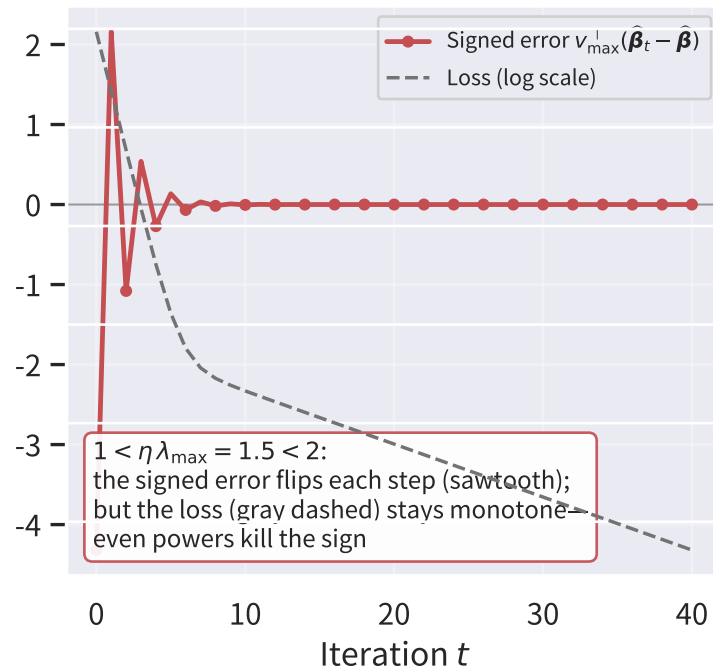
(b) Oscillating decrease: \eta = 1.5
