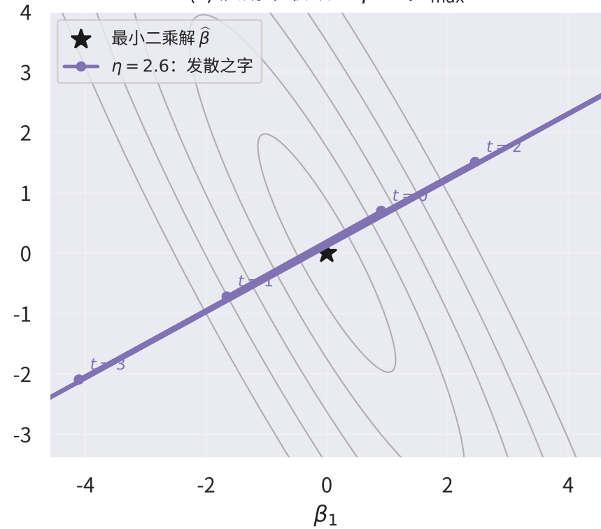
(c) 震荡不收敛: \eta \geq 2/\lambda_{\max}
