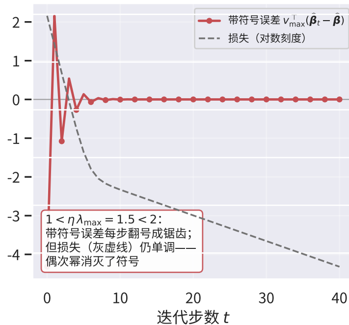
(b) 震荡下降: \eta = 1.5
