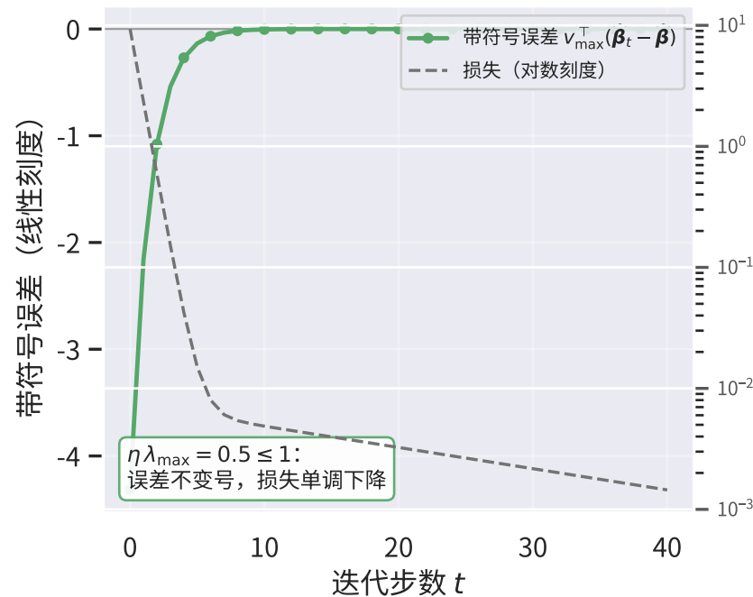
(a) 单调下降: \eta = 0.5
