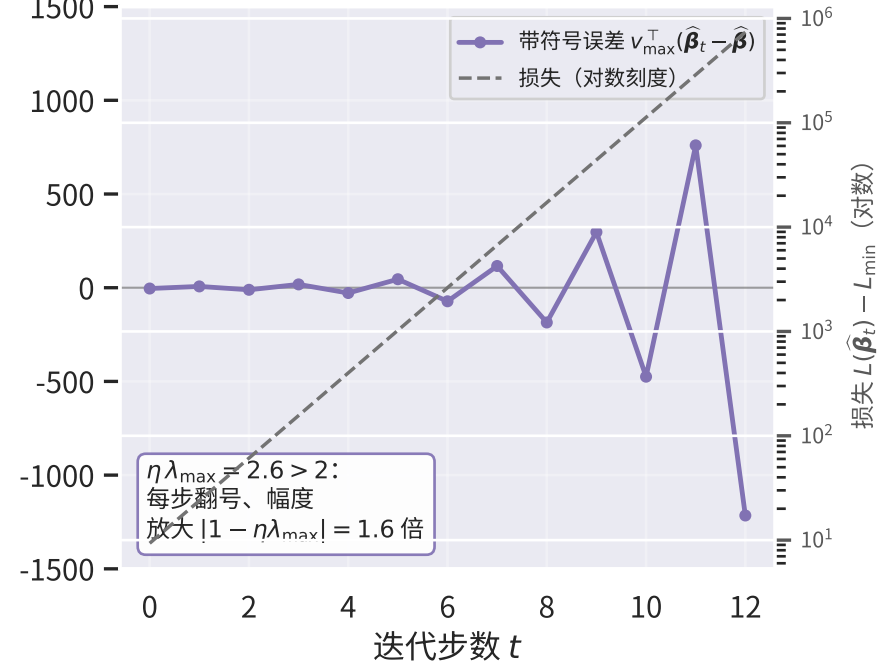
(c) 震荡不收敛: \eta = 2.6
