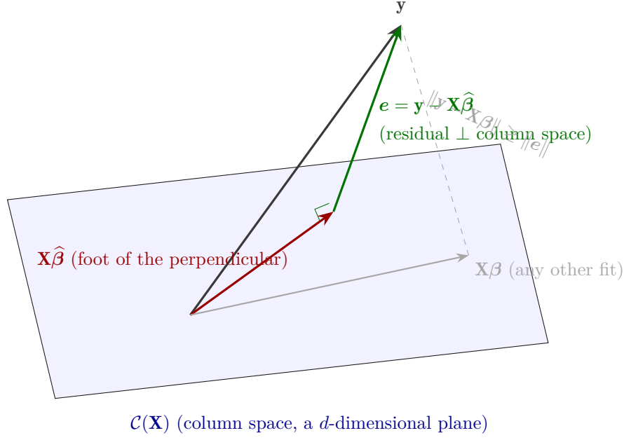
图 4: The geometry of least squares: the foot of the perpendicular from \mathbf{y} to the column space \mathcal{C}(\mathbf{X}) is \mathbf{X}\hat{\boldsymbol{\beta}} . The vertical segment \mathbf{e} is the shortest residual (green); any other fit \mathbf{X}\boldsymbol{\beta} (gray) reaches \mathbf{y} along a longer slanted line —perpendicularity is optimality.
