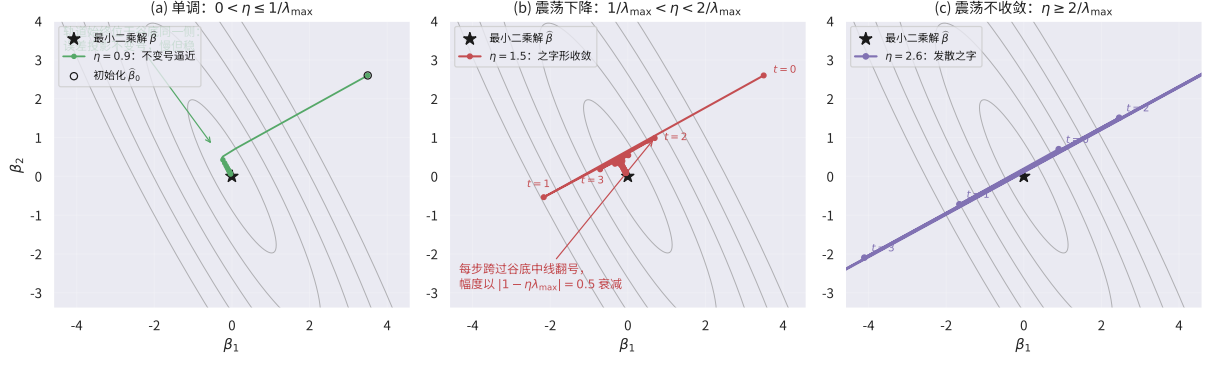
图 6: Three trajectories of gradient descent on a quadratic loss (an elliptical valley with condition number \kappa = 25 ), one per step-size regime: (a) \eta = 0.9 \leq 1/\lambda_{\max} —the trajectory never crosses the valley floor, approaching without sign flips, but crawls slowly along the “thin” direction; (b) 1/\lambda_{\max} < \eta = 1.5 < 2/\lambda_{\max} —the trajectory crosses the valley floor and flips sign every step, the zigzag amplitude decaying by |1 - \eta\lambda_{\max}| = 0.5 —oscillating descent; (c) \eta = 2.6 > 2/\lambda_{\max} —every step flips sign with amplitude growing by 1.6, flying out of view within a few steps.
