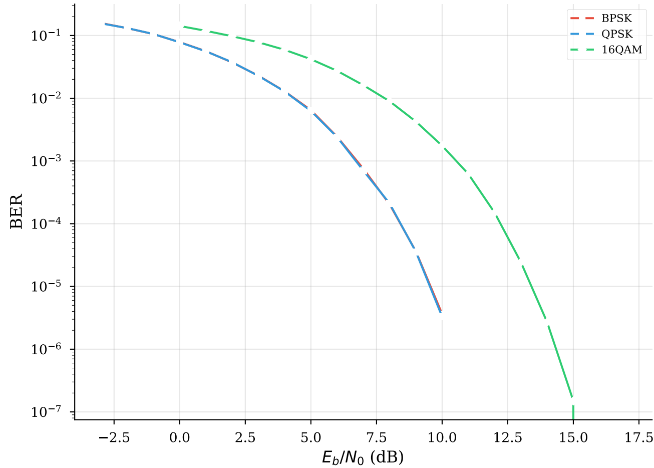
(a) Multi-Modulation BER (AWGN)
