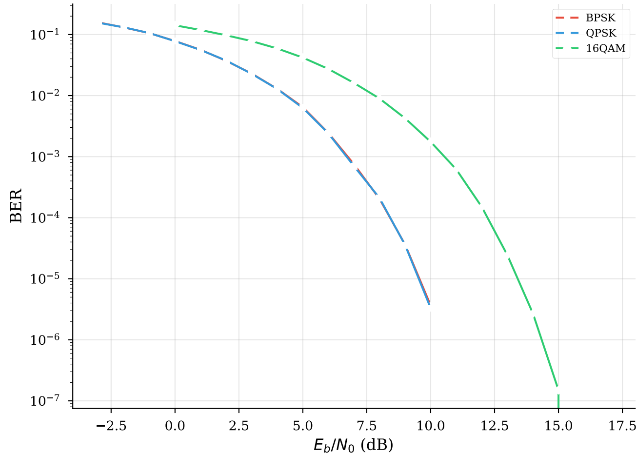
(a) Multi-Modulation BER (AWGN)
