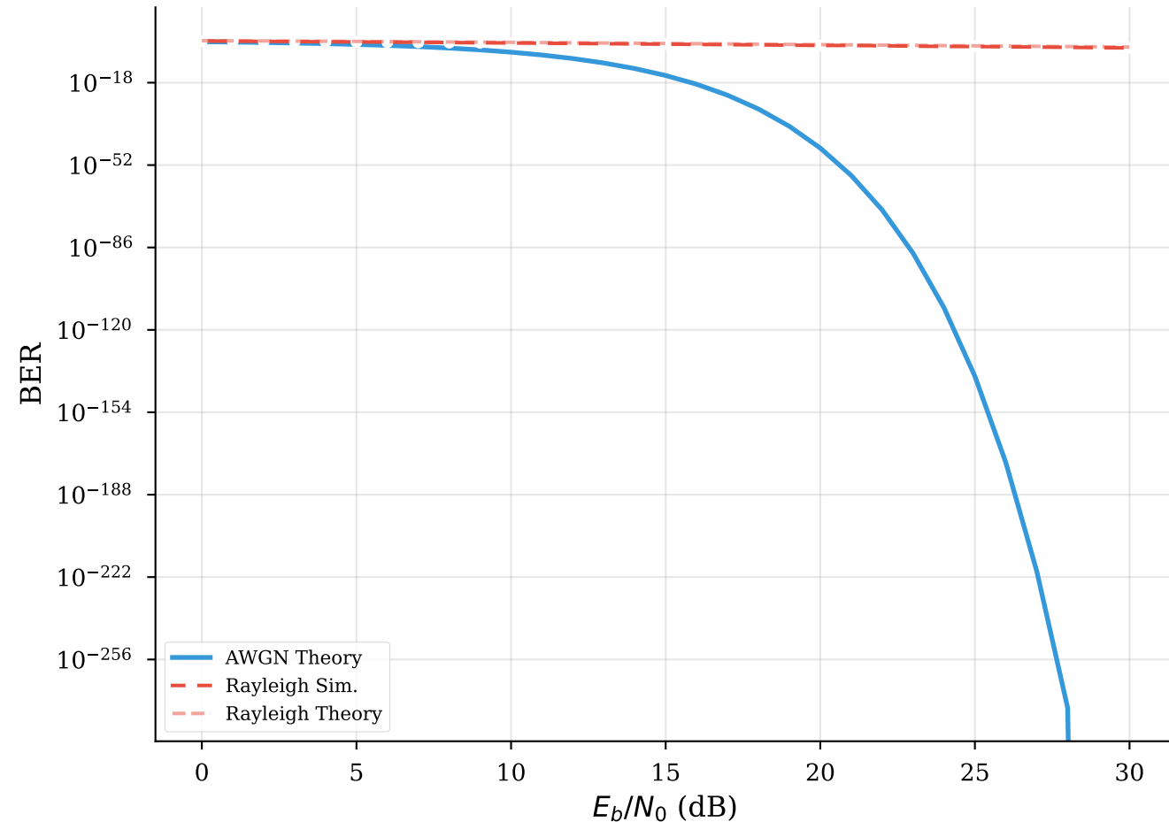
(b) AWGN vs Rayleigh Fading
