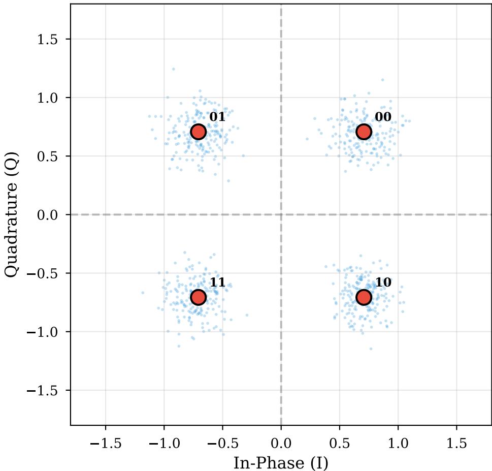
(c) QPSK Constellation (with noise samples)
