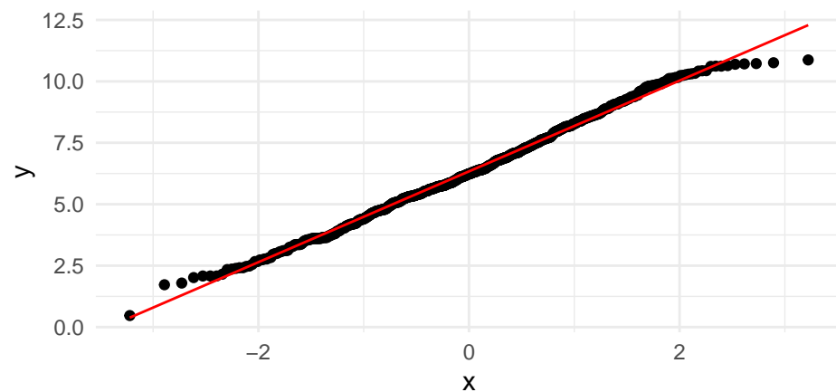
Q-Q Plot (Sqrt)
