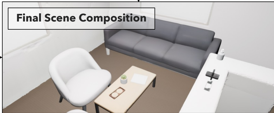
FIRE3D-Shape Network
