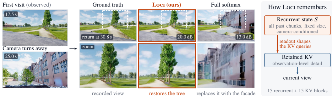
Figure 1: Returning to a previously seen place. Both models receive the recorded video up to 17.75s and the camera trajectory, then generate the rest with full history. At the return (30.8s), a full-softmax model trained with the same backbone, data and recipe replaces the tree with the facade observed in between; Loci restores it (PSNR against ground truth; bottom row: dashed region). Right: Loci keeps a camera-conditioned recurrent state over all past chunks, and its readout shapes the queries with which later blocks attend to retained key-value features.
