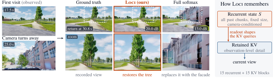
Figure 1: Returning to a previously seen place. Both models receive the recorded video up to 17.75 s and the camera trajectory, then generate the rest with full history. At the return (30.8 s), a full-softmax model trained with the same backbone, data and recipe replaces the tree with the facade observed in between; LocI restores it (PSNR against ground truth; bottom row: dashed region). Right: LocI keeps a camera-conditioned recurrent state over all past chunks, and its readout shapes the queries with which later blocks attend to retained key–value features.
