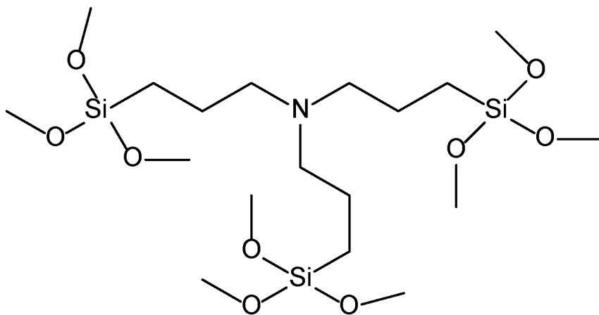
- 3-(Triethoxysilyl)-N,N-bis[3-(triethoxysilyl)propyl]-1-propanamin
