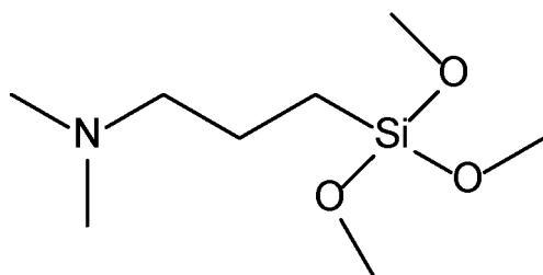
- (2-Dimethylaminoethyl)triethoxysilan.
