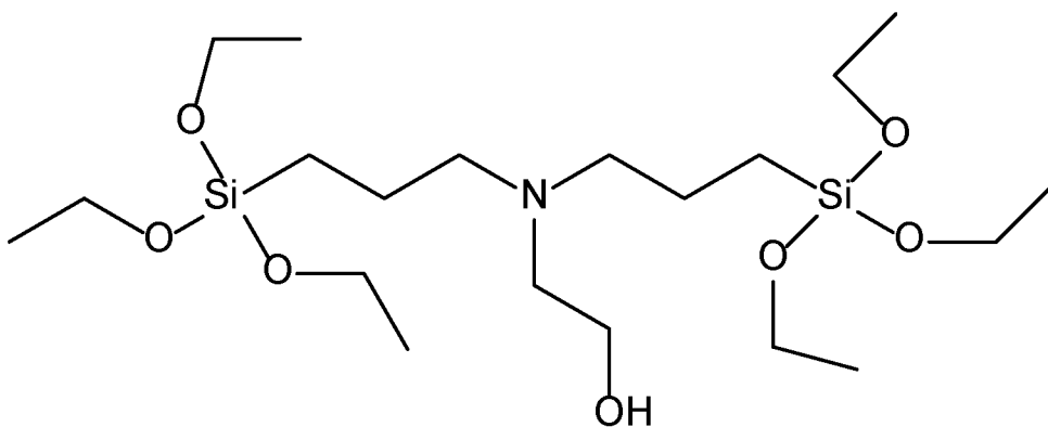
- 3-(Trimethoxysilyl)-N,N-bis[3-(trimethoxysilyl)propyl]-1-propanamin
