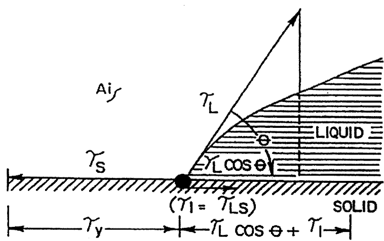
FIG. 2 Prior Art
