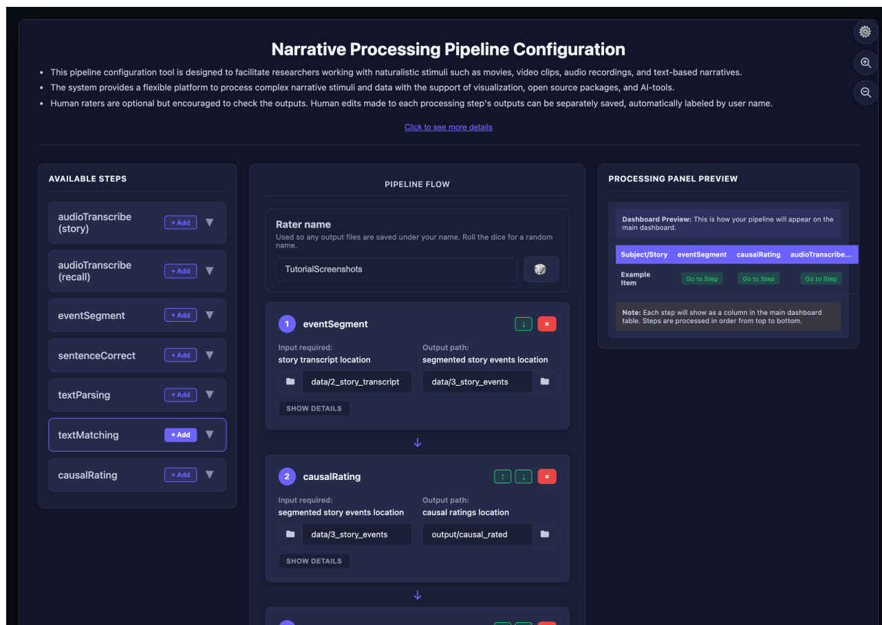
Figure 2: Pipeline configuration builder -- drag steps from the 'Available Steps' palette on the left into the 'Pipeline Flow' canvas in the middle. The Rater name box and dice sit at the top of that middle panel.
