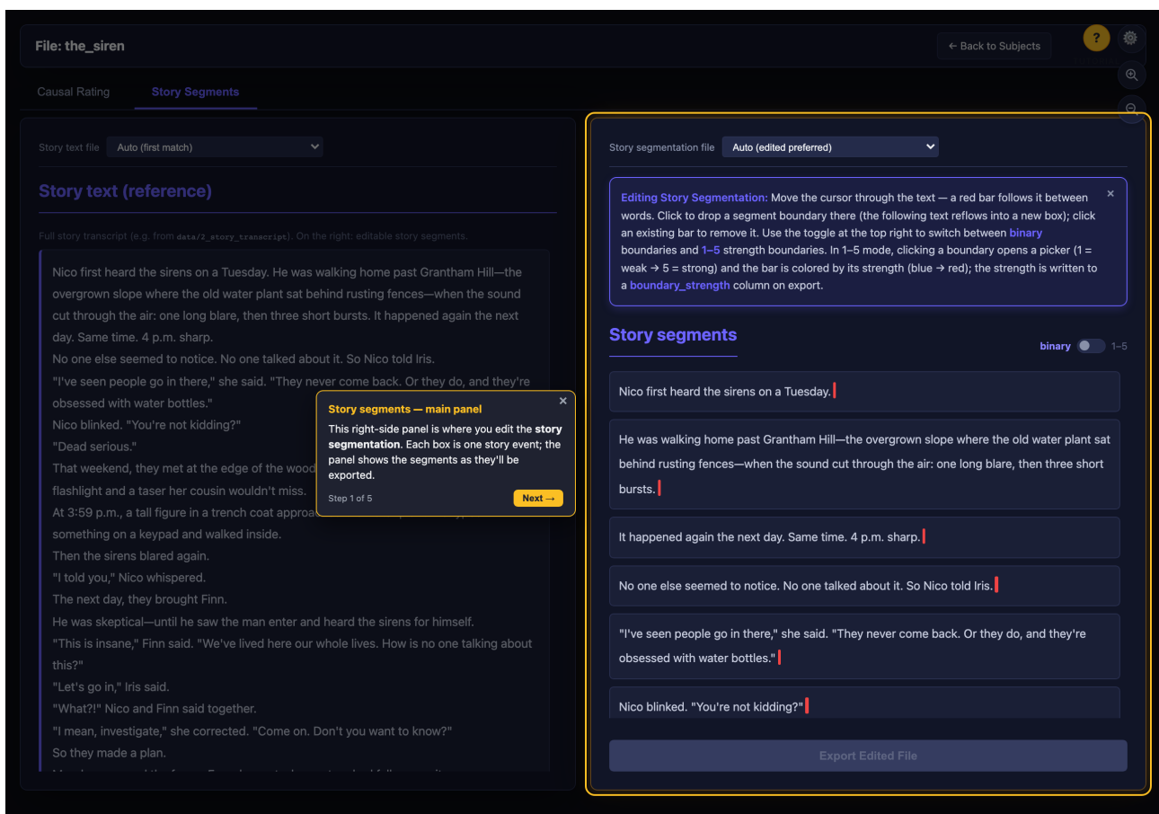
Figure: the interactive walkthrough running on the Story Segments tab -- the spotlight highlights the panel being explained while the rest of the page is
