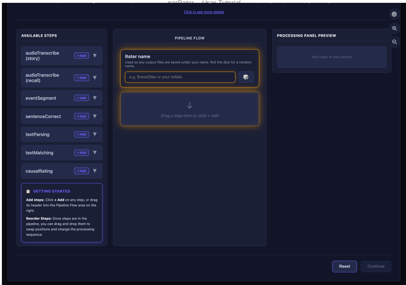
Figure 1: Pipeline Configuration -- the Rater name box (with the dice button) sits at the top of the Pipeline Flow panel in the middle. The Continue button stays greyed out until a rater name is entered AND at least one step has been added.
