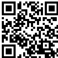
DLSRL
