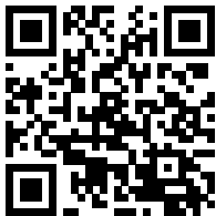
OptGraph
