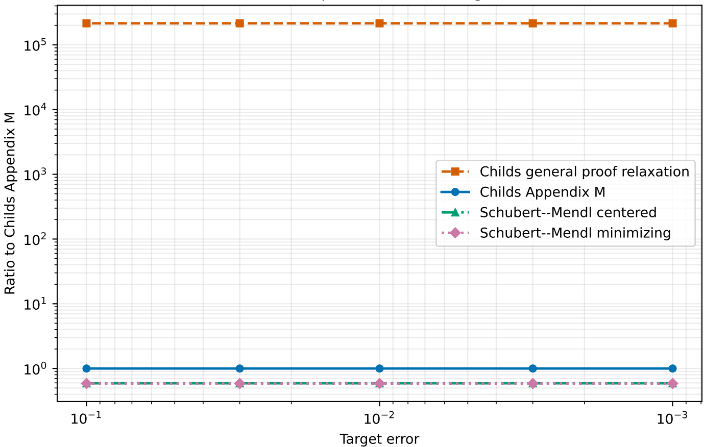
Fourth-order bound comparison: heisenberg chain (multi-term)
