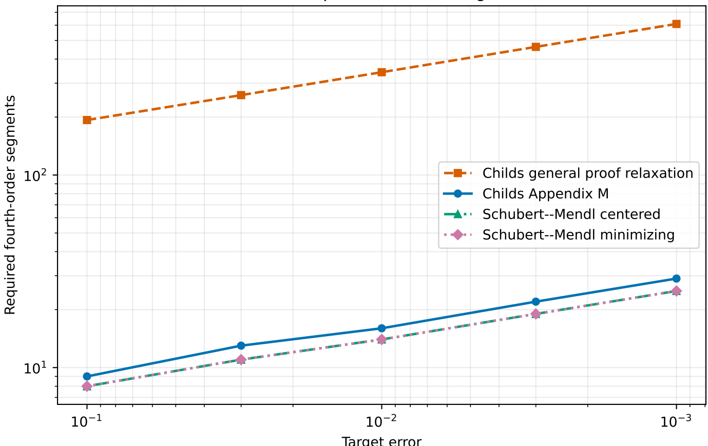
Fourth-order bound comparison: heisenberg chain (multi-term)
