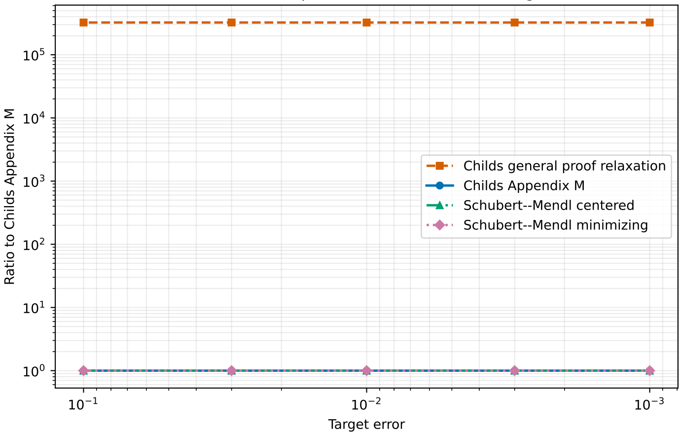
Fourth-order bound comparison: transverse field izing (two-term)
