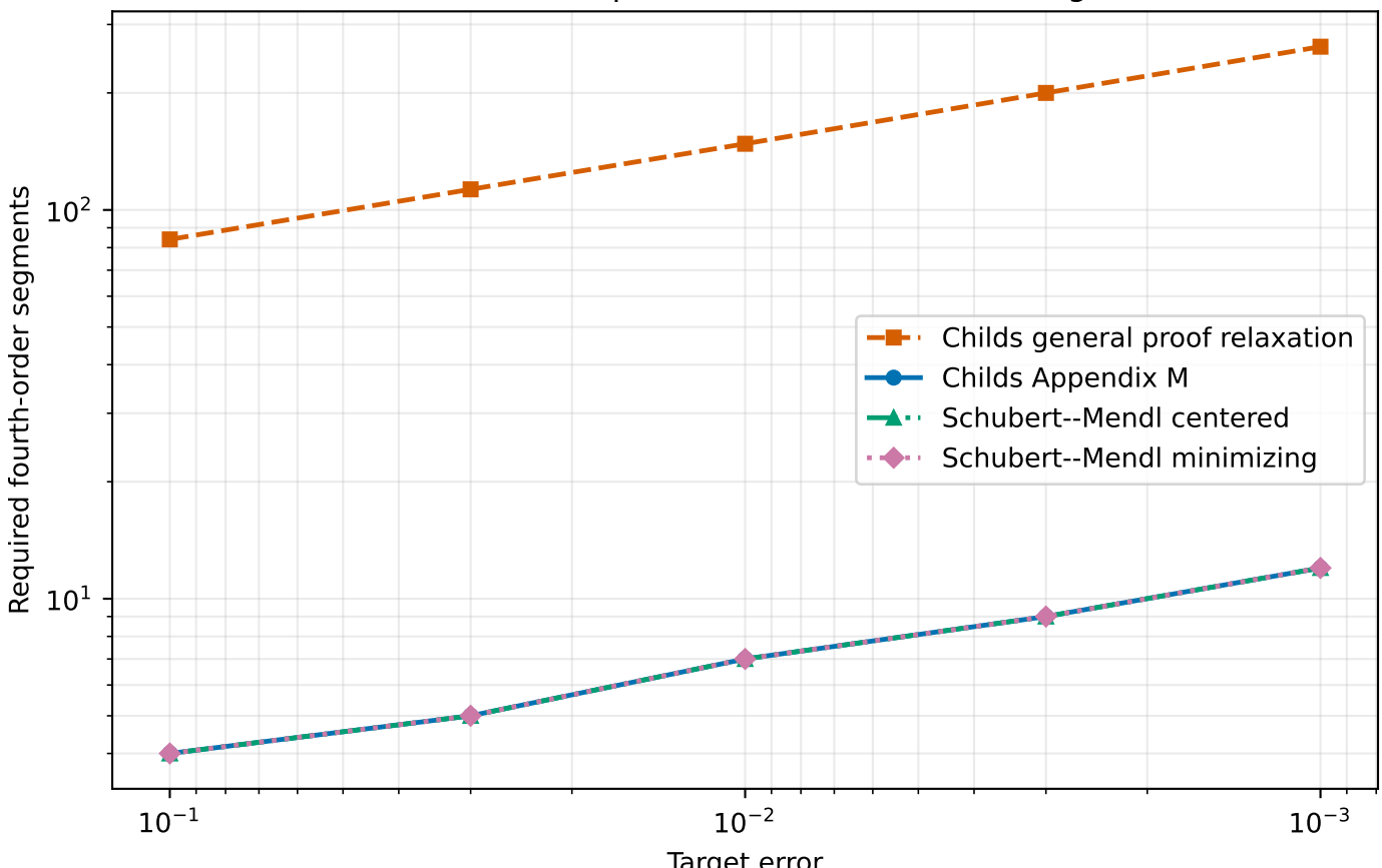
Fourth-order bound comparison: transverse field izing (two-term)
