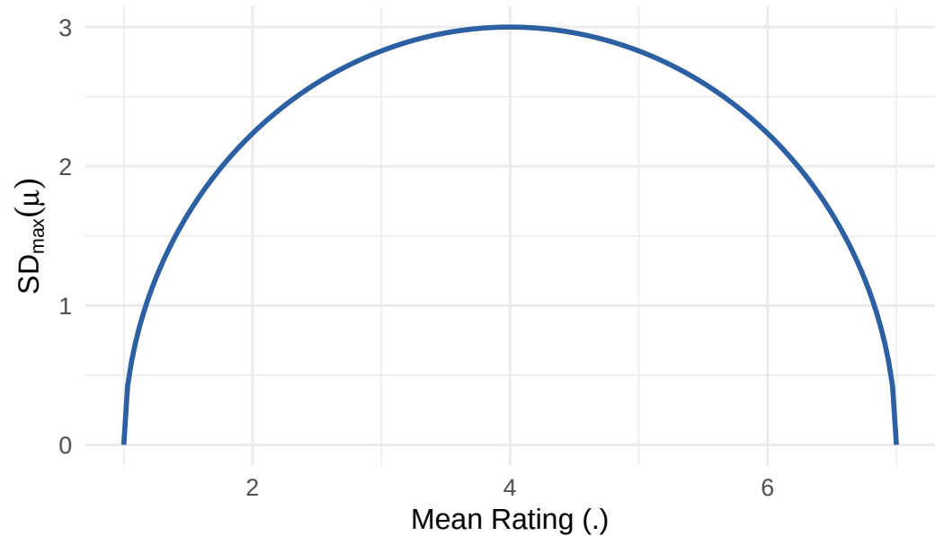
Maximum Possible SD as a Function of the Mean
