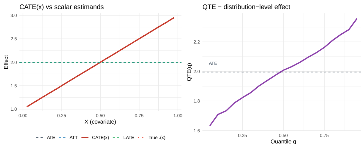
Figure 2.1.: Five views of the same DGP. The horizontal lines for ATE/ATT/LATE collapse the effect to a single scalar. CATE(x) shows how the effect varies with X. QTE(q) shows how the effect varies across the outcome distribution. Each curve answers a different question.
