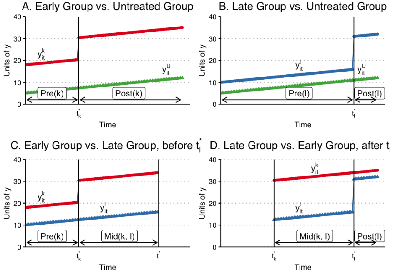
Figure 12.2.: Bacon decomposition
