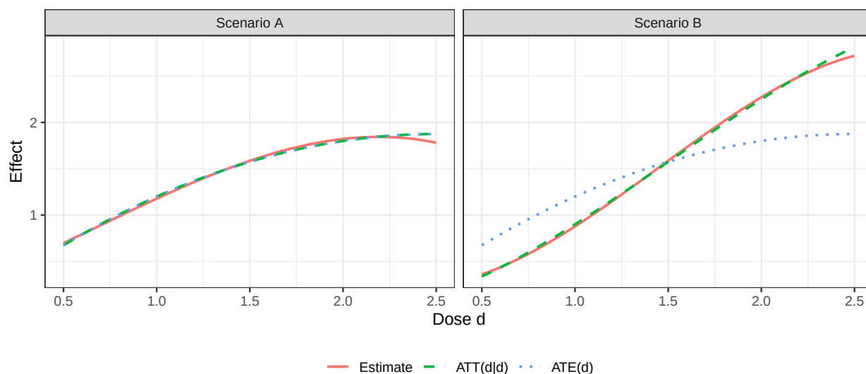
Figure 13.1.: Estimated dose-response curve against the true ATT(d|d) and ATE(d) . In scenario A the two truths coincide.
