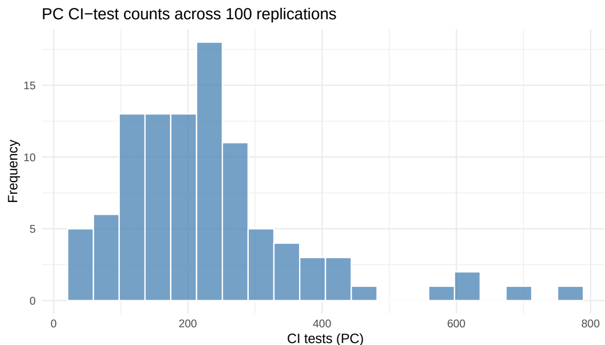
Figure 20.3.: Distribution of PC's CI-test counts across 100 replications. The spread reflects how PC's cost depends on the realized graph density and the order of CI decisions.
