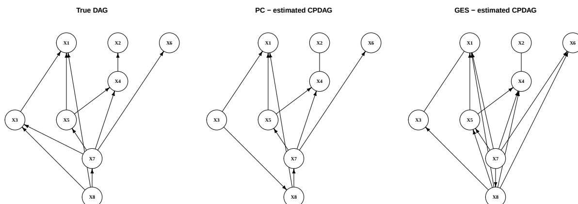
Figure 20.2.: True DAG vs. estimated CPDAGs. Arrows denote oriented edges; lines without arrowheads are unoriented (both directions are CI-equivalent).
