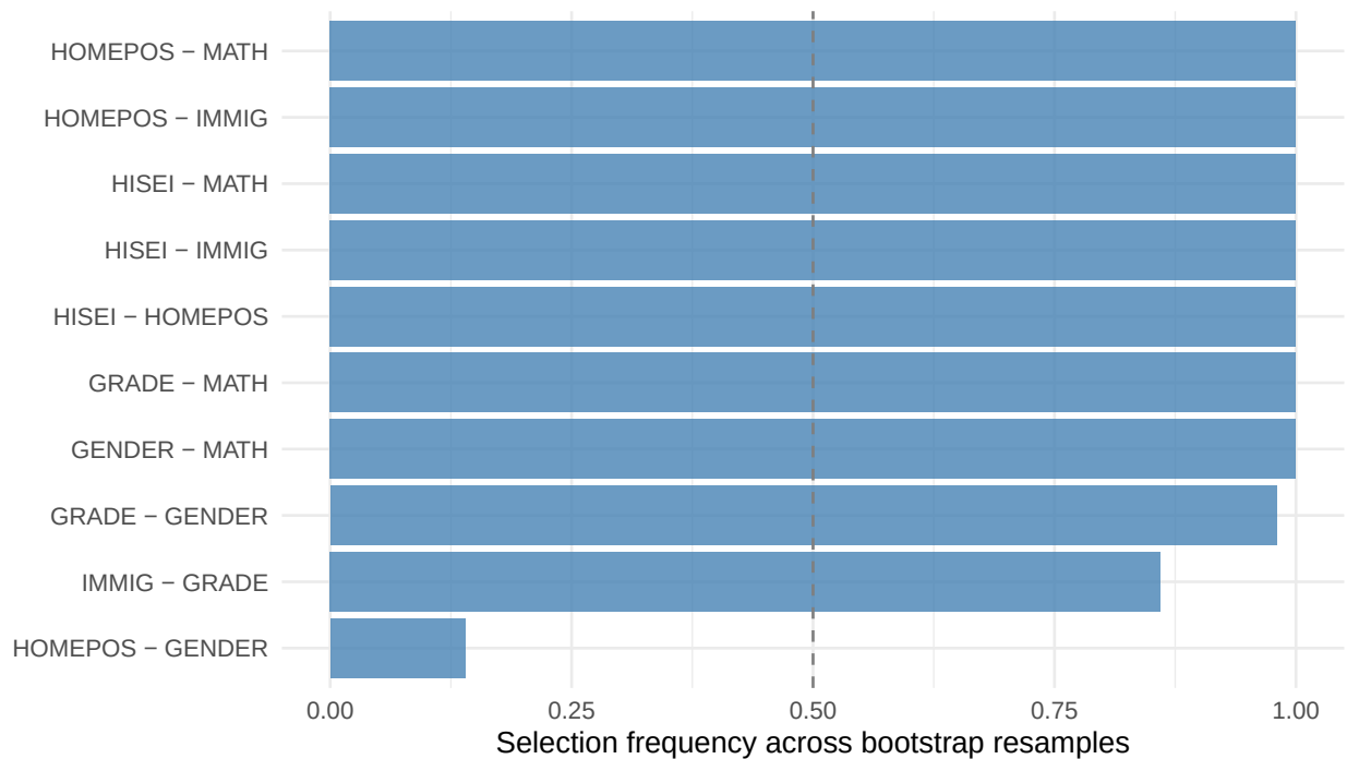
Figure 20.6.: Bootstrap edge-selection frequency (weighted PC, 200 resamples). Edges near 1.0 are robust; near 0.5 are sample-dependent.
