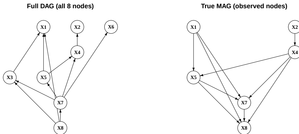
Figure 21.1.: Full DAG (all 8 nodes) and the true MAG skeleton over observed variables. The MAG skeleton includes both direct paths and paths through hidden nodes.
