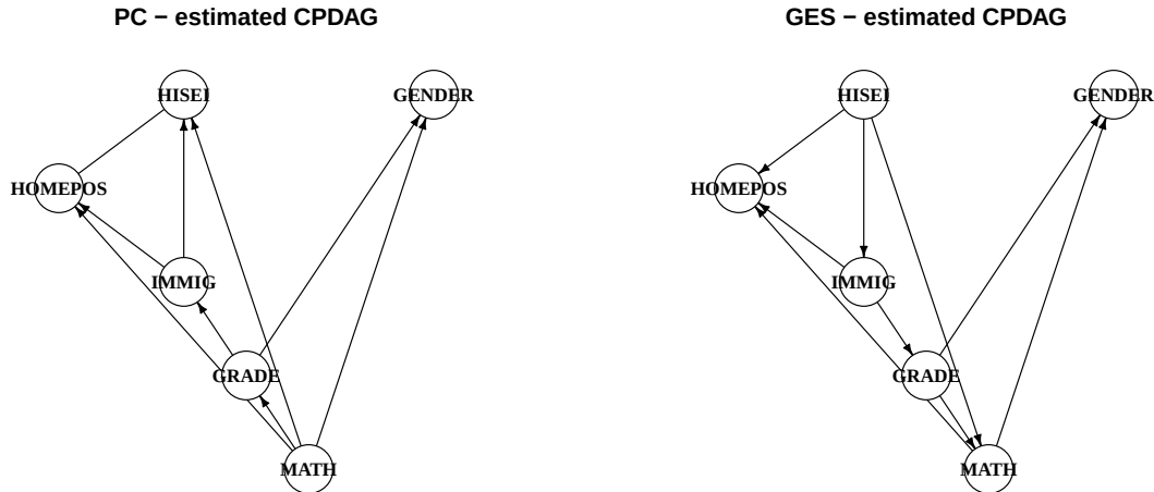
Figure 20.4.: Estimated CPDAGs from PC and GES on PISA 2022 (USA). Arrows are oriented edges; plain lines are unoriented. There is no true-DAG panel — on real data we have no ground truth.
