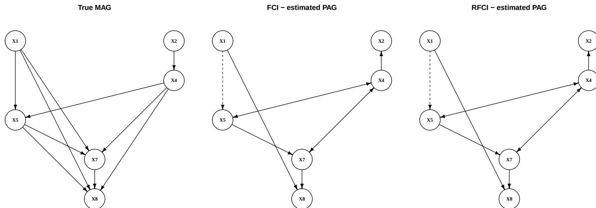
Figure 21.3.: True MAG vs. PAGs recovered by FCI and RFCI. Directed arrows are definite cause-to-effect; bidirected ( ) edges flag hidden common causes; circle ( ) marks indicate orientations the algorithm could not resolve. RFCI typically leaves more circles than FCI because its orientation phase is deliberately more conservative.
