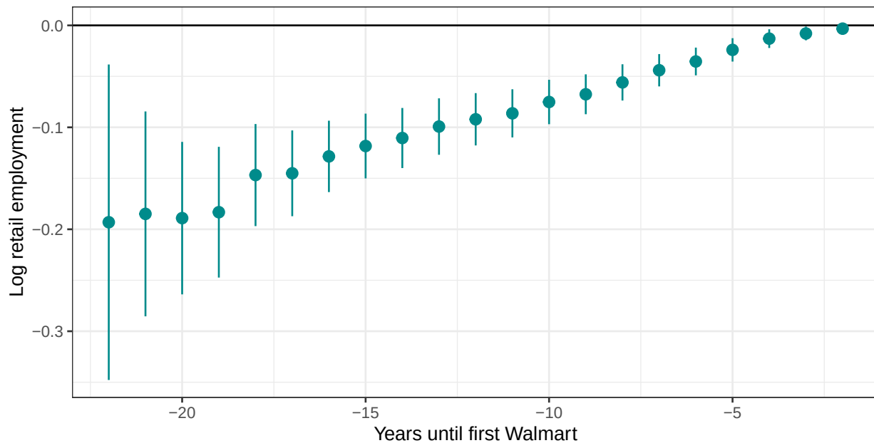
Figure 13.2.: Weighted pre-treatment estimates from the untreated observations, with 95% intervals. The year before entry is the base.
