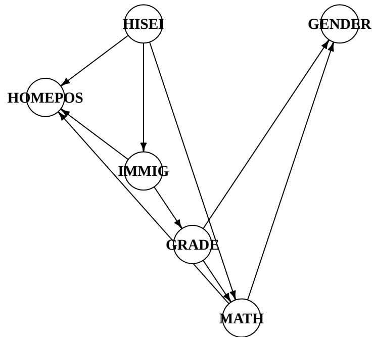
GES – estimated CPDAG
