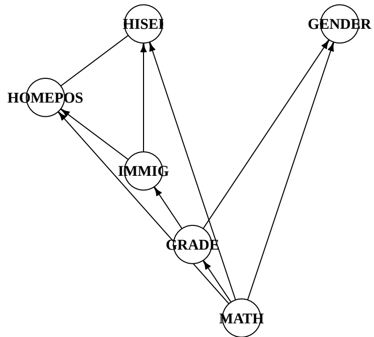
PC – estimated CPDAG
