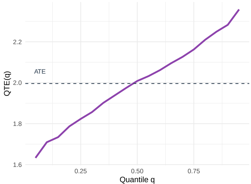
QTE – distribution–level effect
