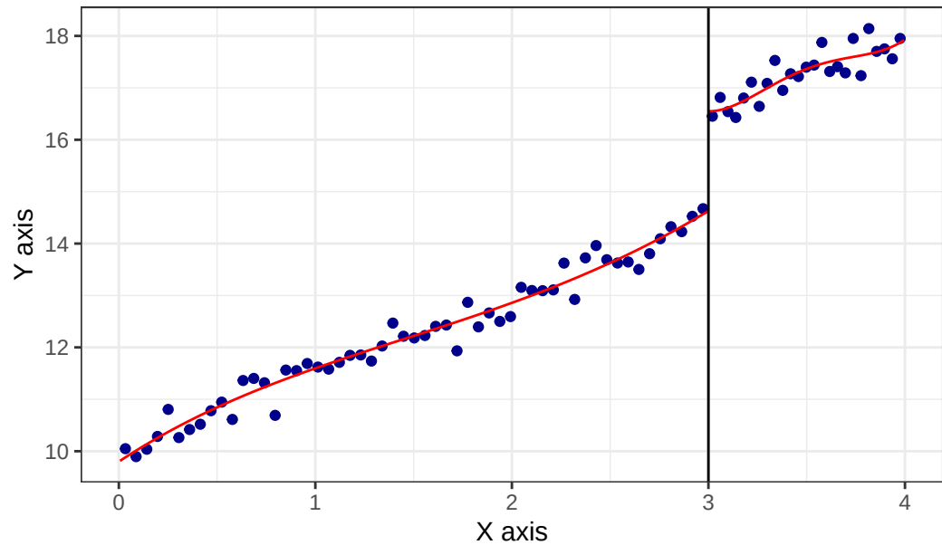
RD Plot
