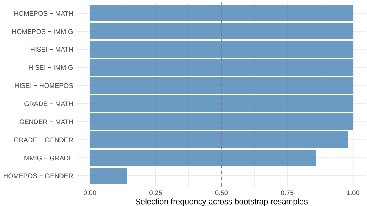
Figure 21.6.: Bootstrap edge-selection frequency (weighted PC, 200 resamples). Edges near 1.0 are robust; near 0.5 are sample-dependent.
