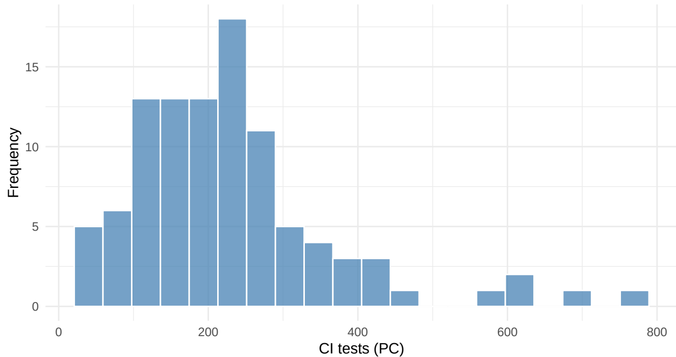
PC CI-test counts across 100 replications
