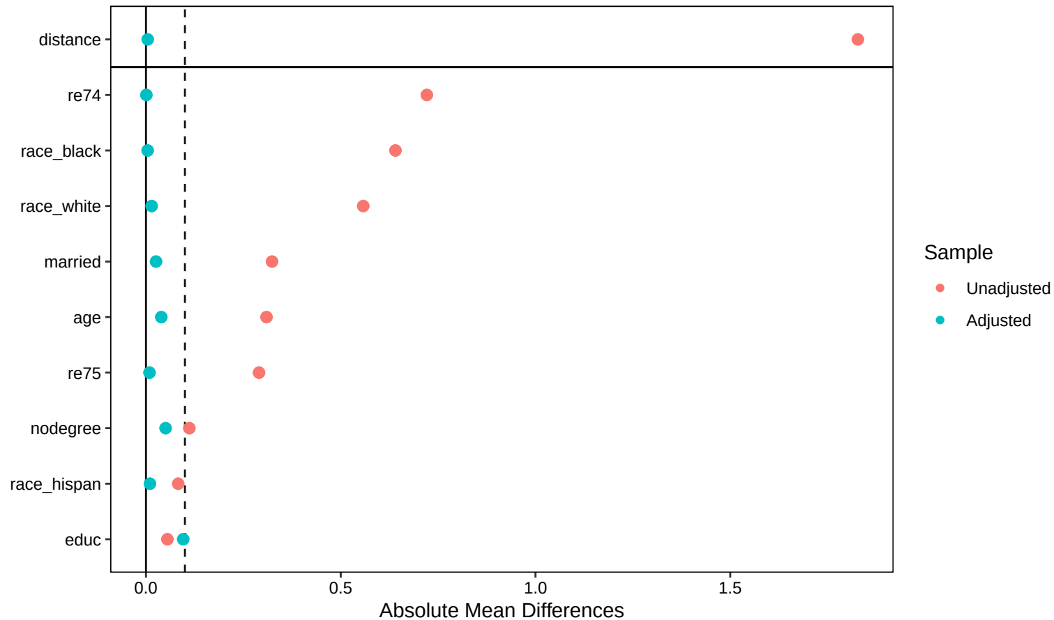
Balance plot – Full matching
