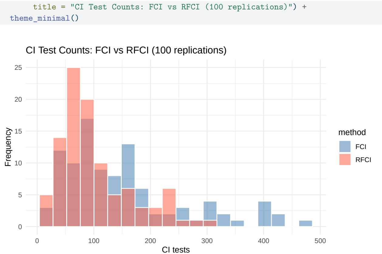
Figure 20.4.: CI-test count distributions across 100 replications. By skipping the Possible-D-SEP tests, RFCI typically — though not always — runs fewer tests than FCI.
