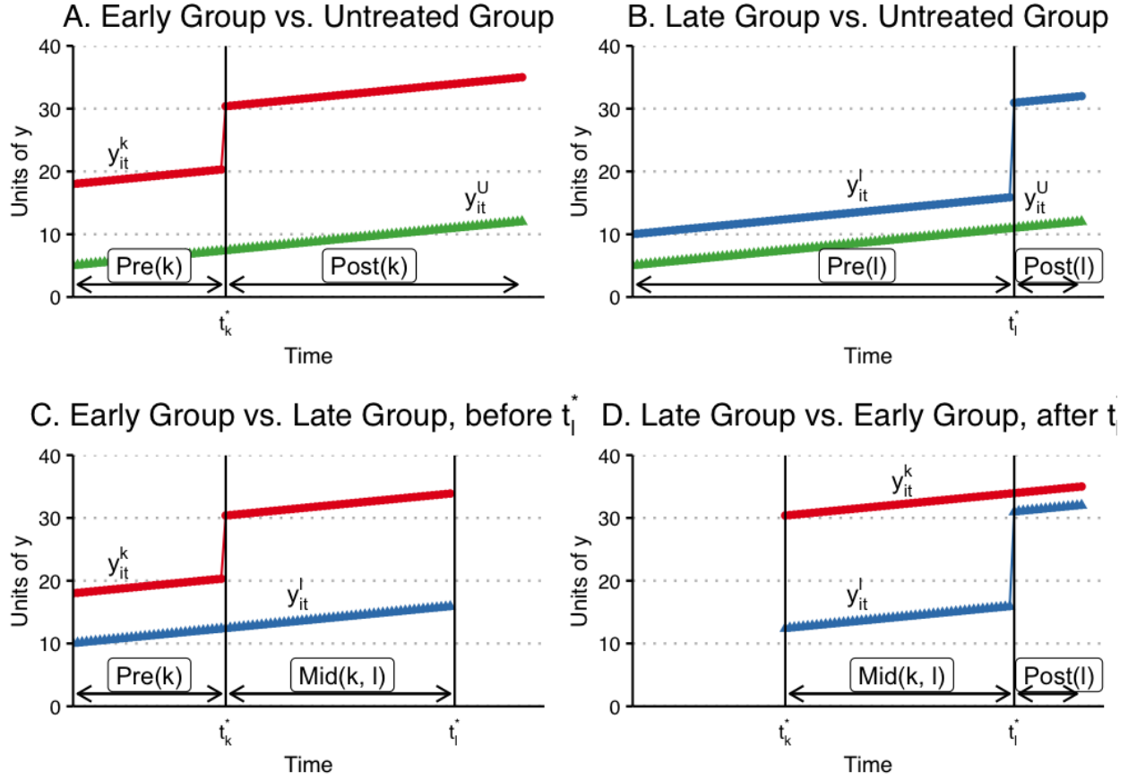
Figure 13.2.: Bacon decomposition
