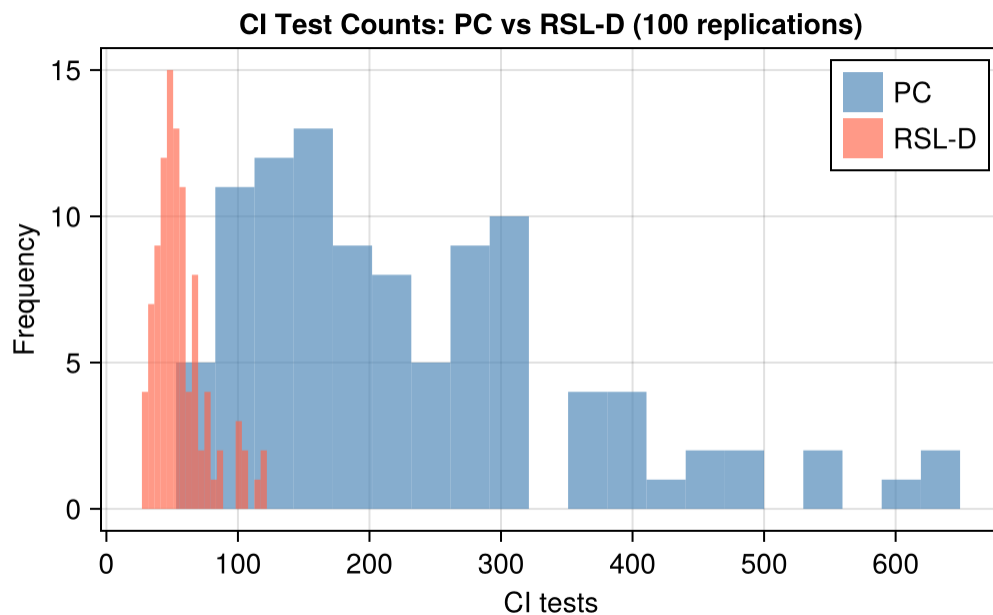
Figure 24.3.: Distribution of CI test counts over 100 replications. RSL-D consistently uses fewer CI tests.
