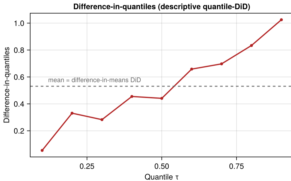
Figure 12.2.: Difference-in-quantiles (a descriptive quantile-DiD), computed at each quantile. This is not an identified QTE: reading it as one needs both an assumption identifying the untreated post-treatment distribution for treated units and a rank condition such as rank invariance. Its average, by contrast, is the ordinary difference-in-means DiD – averaging a quantile function returns a mean – so the information the curve adds is its shape, not its level.
