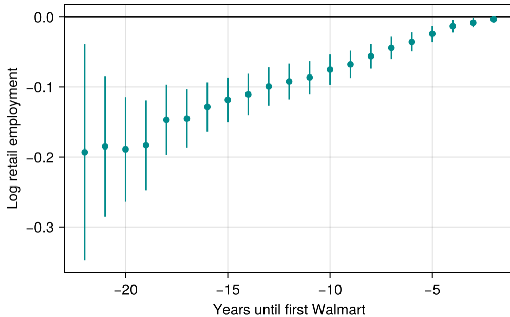
Figure 14.1.: Weighted pre-treatment estimates from the untreated observations, with 95% intervals. The year before entry is the base.
