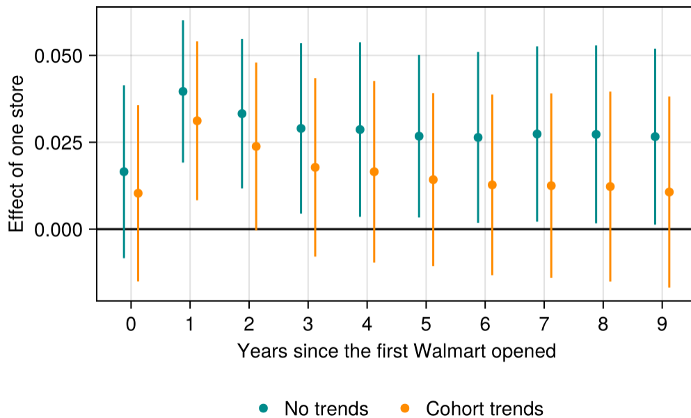
Figure 14.2.: Effect of one Walmart on log retail employment in the 1990 cohort, by year since entry, with 95% intervals.
