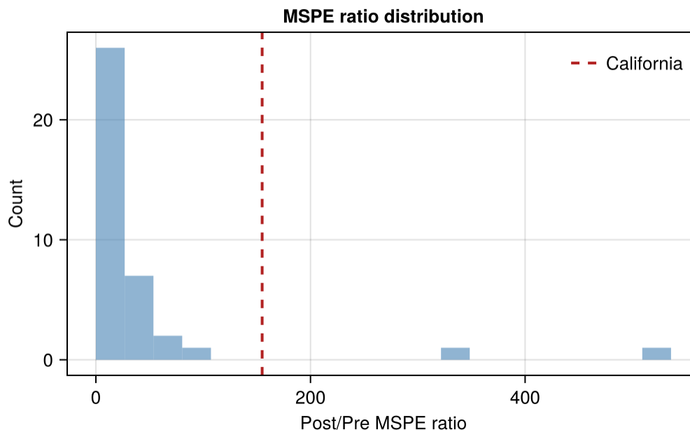
Figure 16.2.: Distribution of post/pre MSPE ratios across donor states (histogram). California's ratio is the red dashed line.
