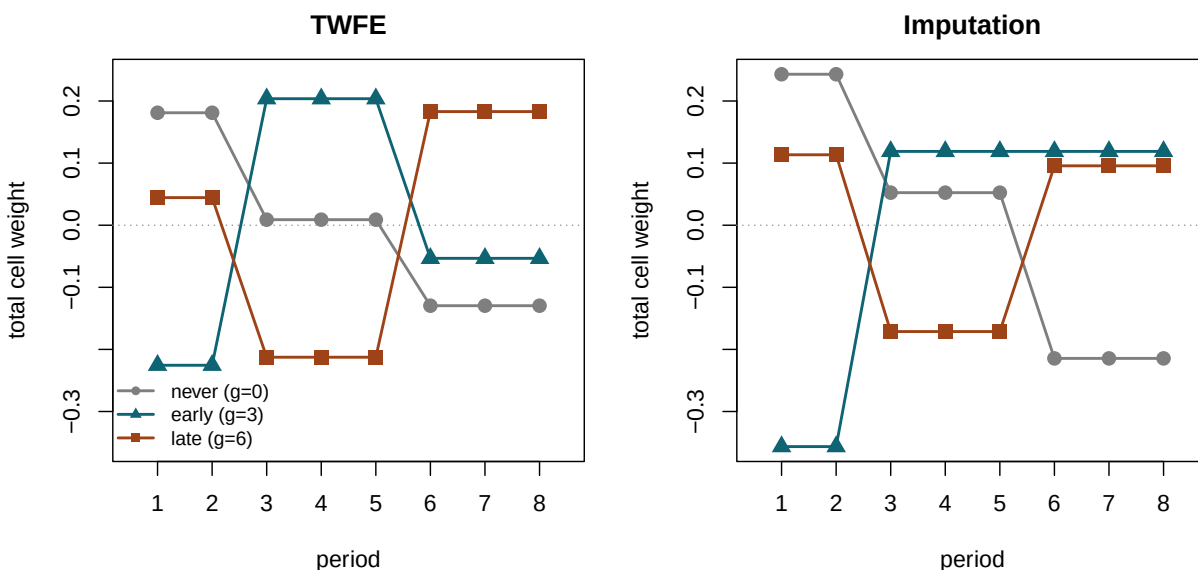
Figure 14.6: Cell-level outcome weights in the staggered panel, summed within each cohort-period cell. TWFE (left): the early cohort's treated cells (teal triangles) turn negative in periods 6–8 — those outcomes are subtracted from \hat{\beta} , the observation-level signature of the forbidden comparison. Imputation (right): every treated cell stays positive; no treated observation can count as a control.
