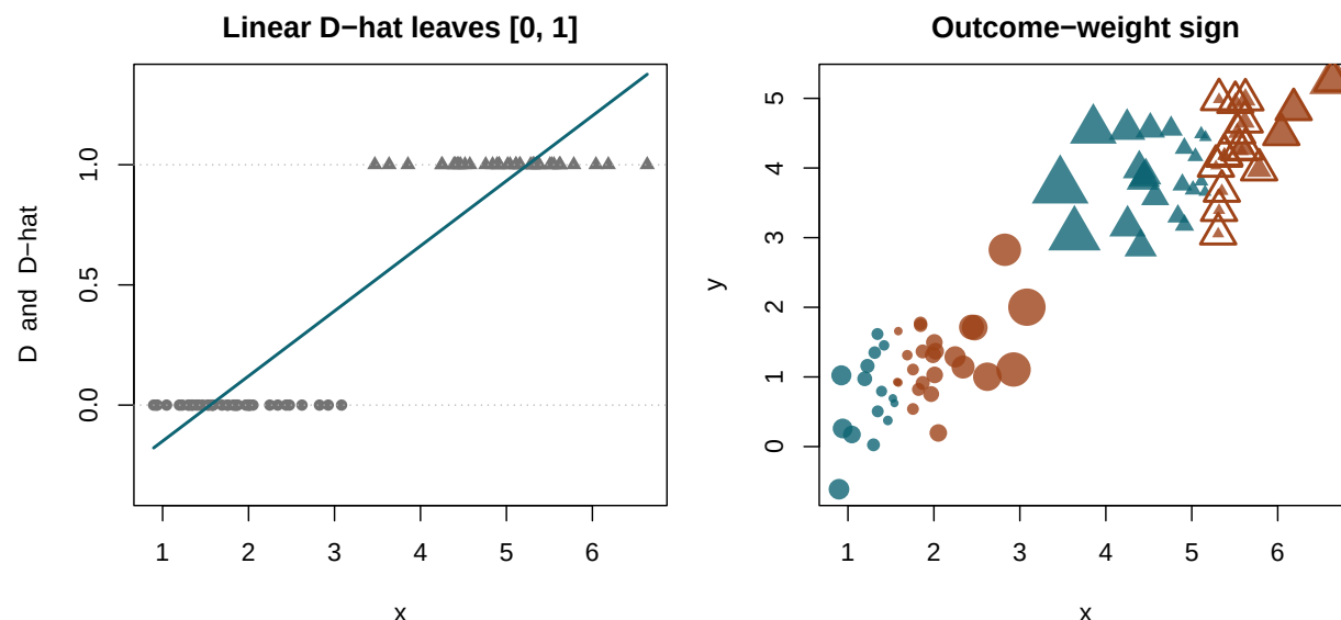
Figure 14.2: Outcome weights under thin overlap. Left: the linear projection \hat{D} of treatment on x leaves [0, 1] , so residuals change sign in the extrapolation zone. Right: outcome weights coloured by sign (teal +, rust −), triangles treated and circles control, size \propto |\omega_i| . Treated units at high x (open rust triangles) carry negative weights — their outcomes are subtracted from \hat{\beta} — a sign the effect weights \tilde{V}_i^2 \geq 0 cannot reveal.
