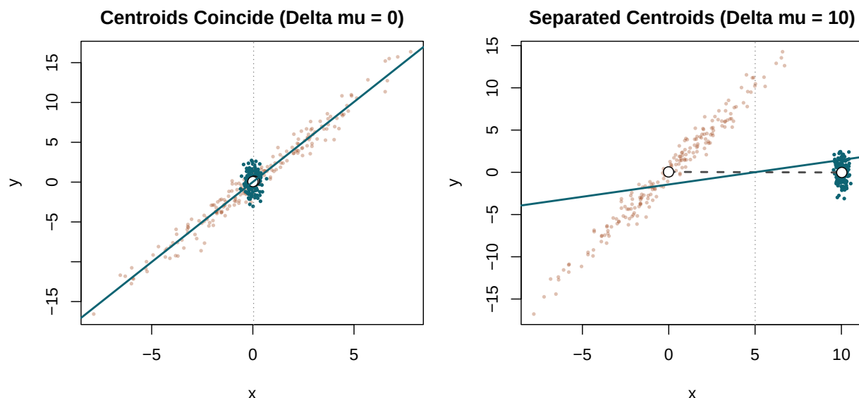
Figure 13.1: Pooled OLS as a within/between blend (Equation 13.29). Points are the two groups, open circles their centroids. The dashed line is the between-slope \beta_{between} = \Delta\bar{y}/\Delta\mu through the centroids; the solid line is the pooled fit \hat{\beta}_{OLS} . The within slopes are identical across panels; widening the centroid gap \Delta\mu (left to right) inflates V_{between} and rotates \hat{\beta}_{OLS} away from \beta_{within} toward \beta_{between} .
