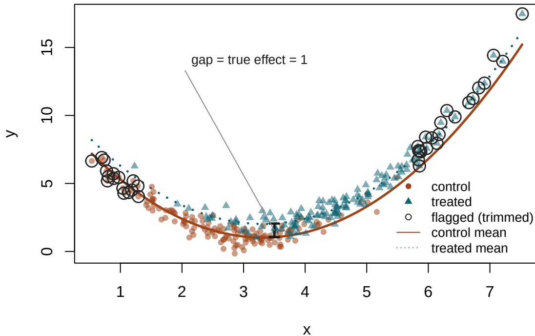
Figure 14.3: A fragile OLS gap. The two curves are the true means — control (rust, solid) and treated (teal, dotted), a constant 1 apart: that gap is the true effect (arrow). Controls sit low on the curve and treated high, so the groups share only the middle. Ringed points are the extrapolating units the one-line rule flags, where the groups do not overlap. Forcing a straight y \sim D + x across the whole range reports \hat{\beta} = 0.69 ; dropping the flagged units, or reweighting to the overlap, restores \approx 1 .
