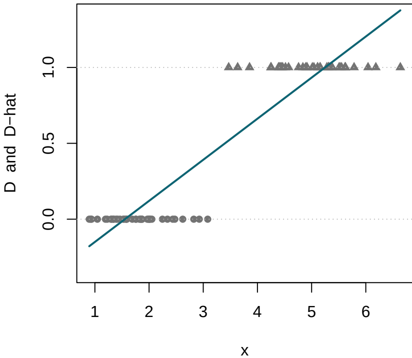
Linear D-hat leaves [0, 1]
