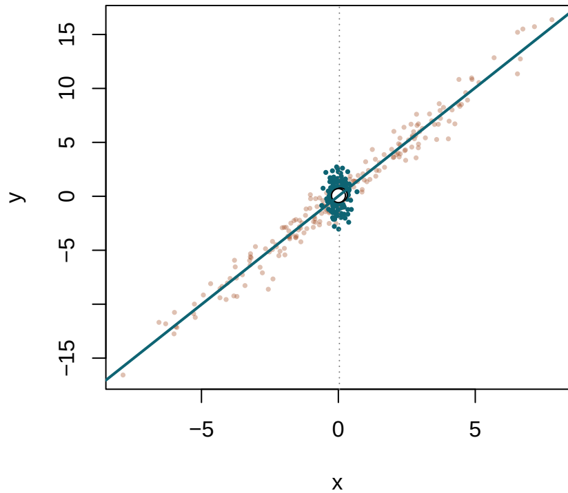
Centroids Coincide (Delta mu = 0)
