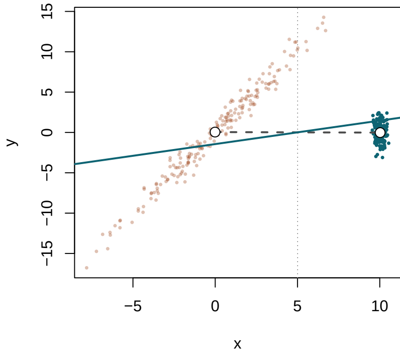
Separated Centroids (Delta mu = 10)
