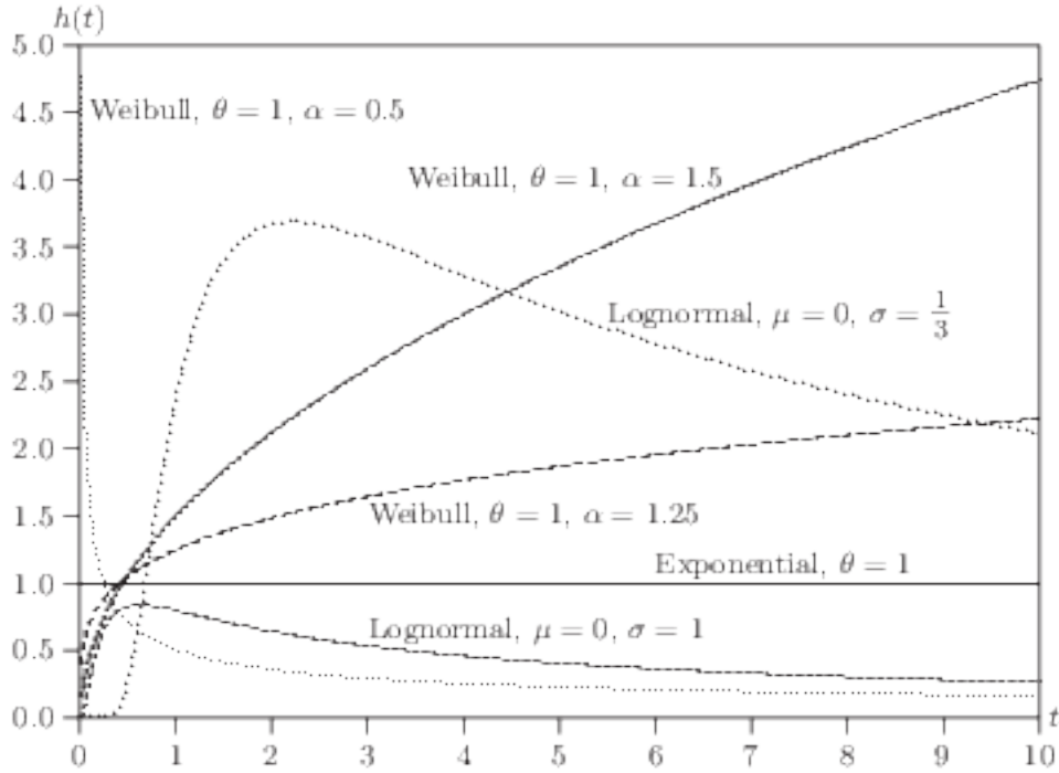
Figure 10.1: Various hazard functions from Davidson and MacKinnon (2004)
