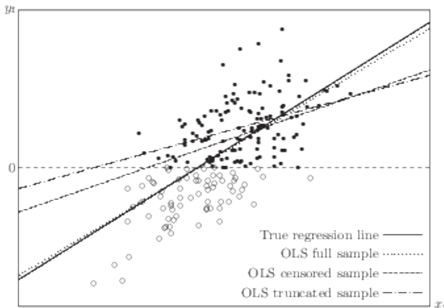
Figure 6.1: Effects of truncation and censoring from Davidson and MacKinnon (2004)
