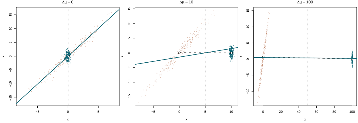
Figure 13.1: Pooled OLS as a within/between blend (Equation 13.18). Points are the two groups, open circles their centroids. The dashed line is the between-slope \beta_{between} = \Delta\bar{y}/\Delta\mu through the centroids; the solid line is the pooled fit \hat{\beta}_{OLS} . The within slopes are identical across panels; widening \Delta\mu (left to right) inflates V_{between} and rotates \hat{\beta}_{OLS} toward \beta_{between} .
