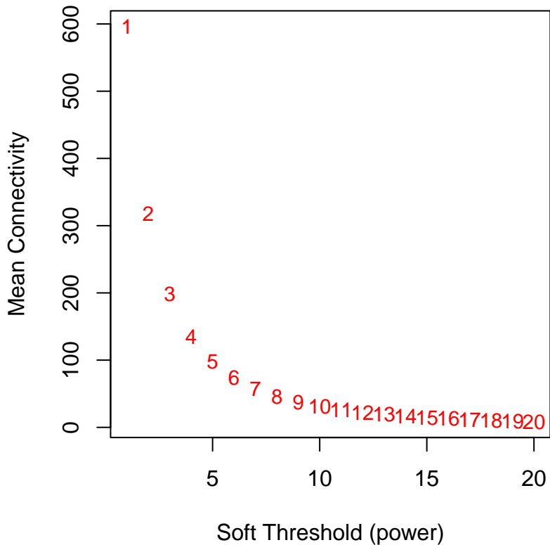
Mean connectivity
