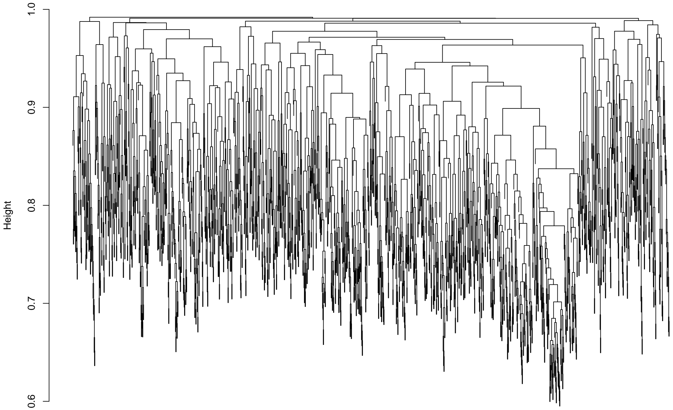
Gene clustering on TOM-based dissimilarity
