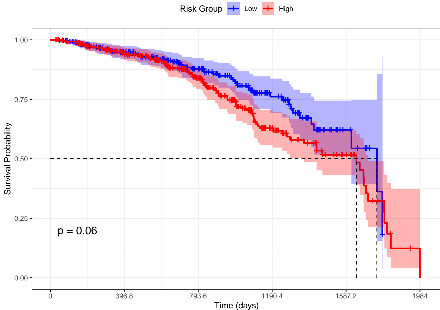
Kaplan–Meier Survival Curve by Risk Group
