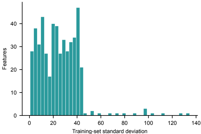
Distribution of feature standard deviations
